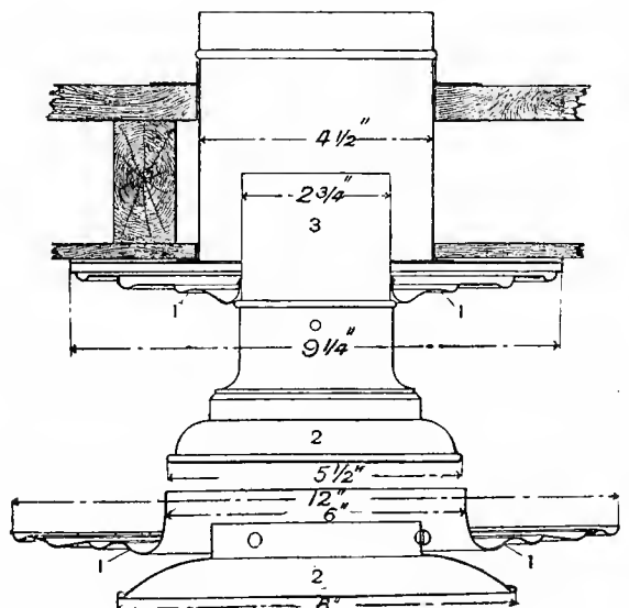
Fig. 3132. CEILING PLATES AND SMOKE-BELL.
